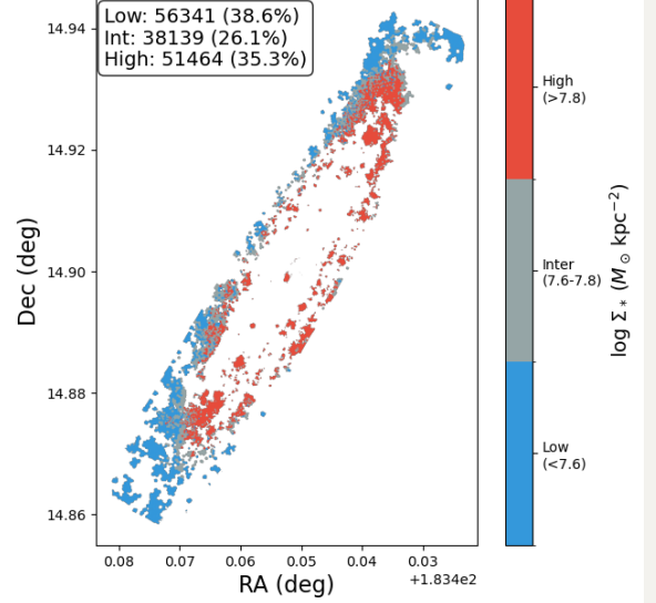
NGC4192: \log \Sigma_{*} Mass Regions
