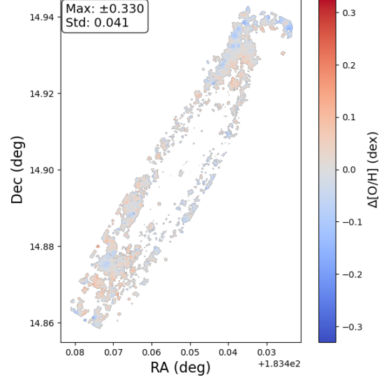
NGC4192: \Delta [\text{O}/\text{H}]_{\text{O3N2} - \text{M13}} (offset from bin average)
