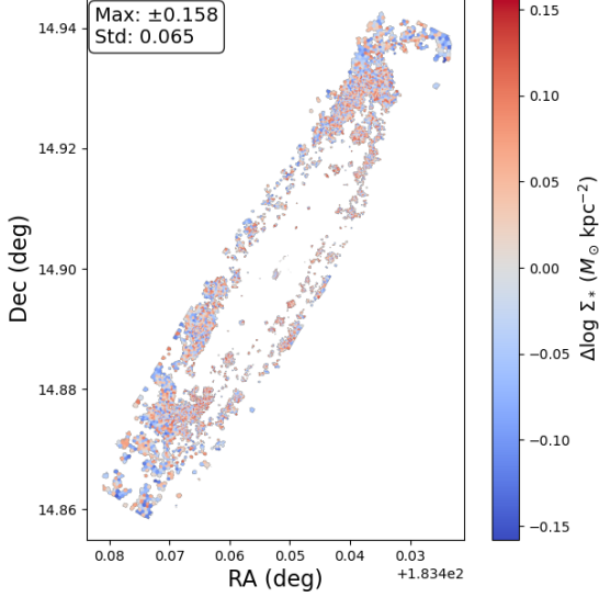
NGC4192: \Delta \log \Sigma_{*} (offset from bin average)
