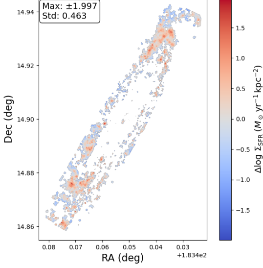
NGC4192: \Delta \log \Sigma_{\text{SFR}} (offset from bin average)
